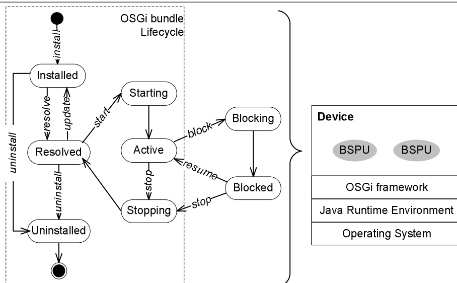
Figure 6.3: Lifecycle of a BSPU which is extended based the component lifecycle in OSGi framework
